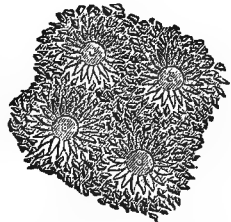
THE SAME, MAGNIFIED
